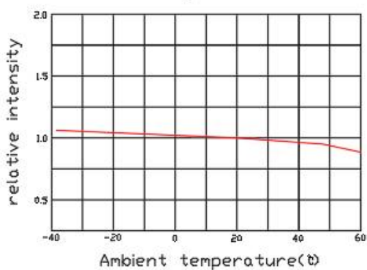
Relative light intensity vs ambient temperature
