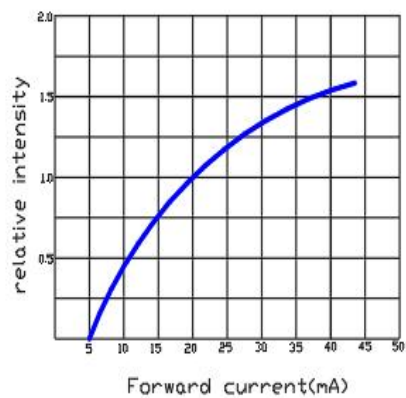
Relative light intensity vs current
