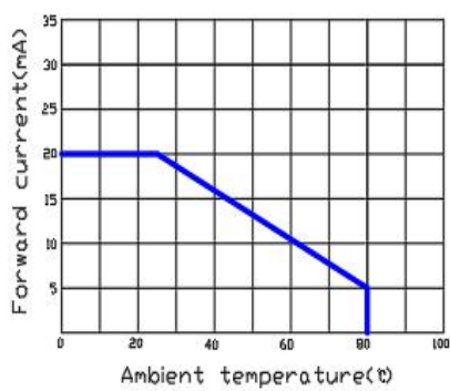
Current and ambient temperature
