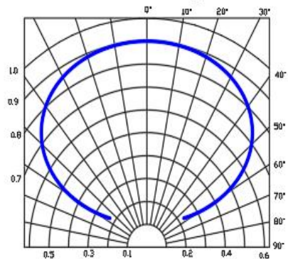
Radiation angle
